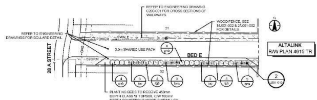
2 WALKWAY PLANTING PLAN SCALE: 1:200
